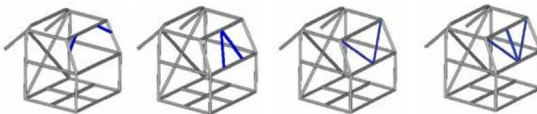
Diagram: Compulsory reinforcement for Buggies
