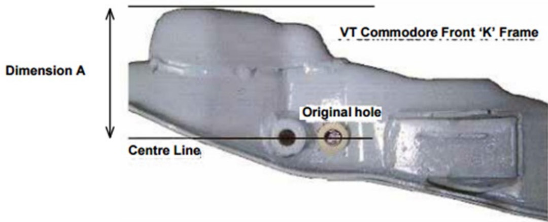
VT Commodore "K" Frame Modification
