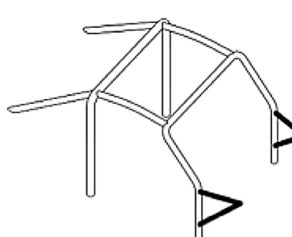
DRAWING J-37
