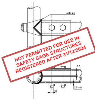
DRAWING J-56
