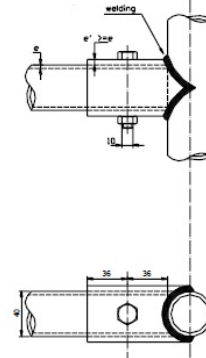
DRAWING J-55
